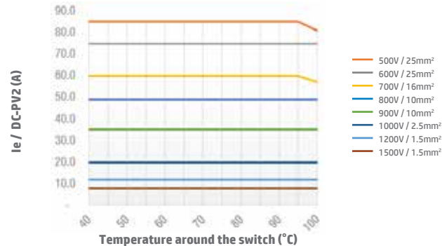
Switch SI55 2H DC-PV2 Open Type
