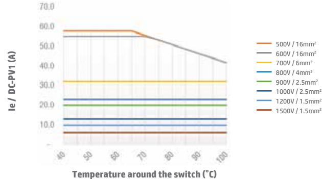
Switch SI32 2H DC-PV1 Open Type
