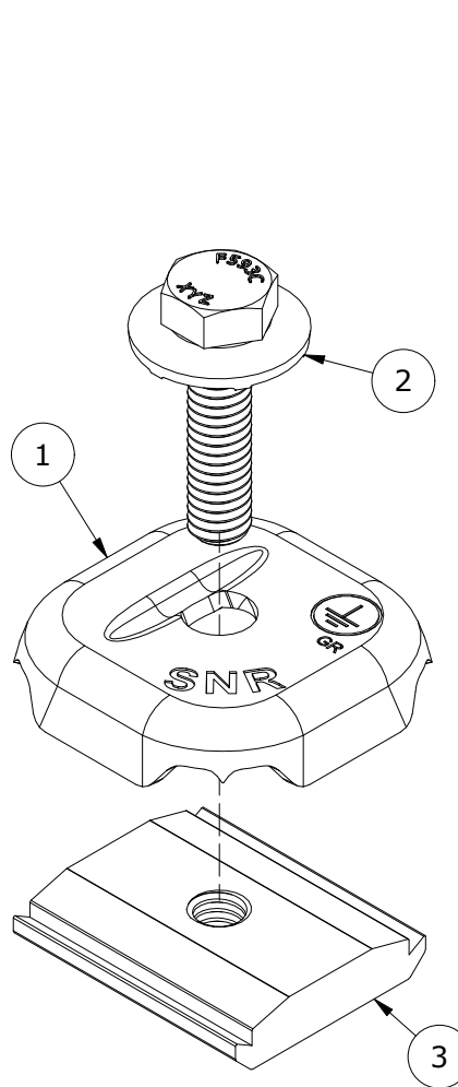
EXPLODED VIEW
