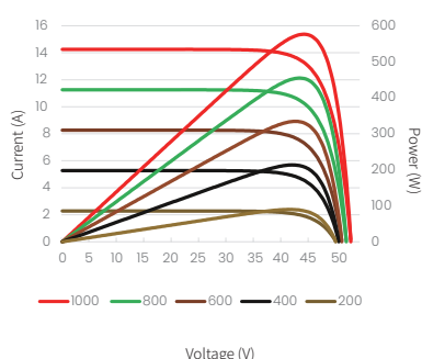
Current-Voltage &amp; Power-Voltage Curves (585W)
