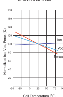
Temperature Dependence of I_{sc} , V_{oc} , P_{max}
