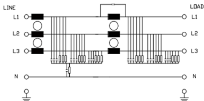
Schematic
