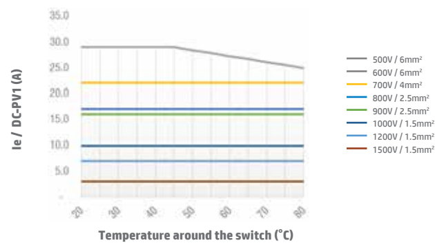
Switch SI16 2H DC-PV1 Enclosed Type
