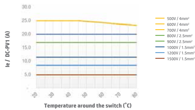
Switch SI25 2 poles DC-PV1 Enclosed Type
