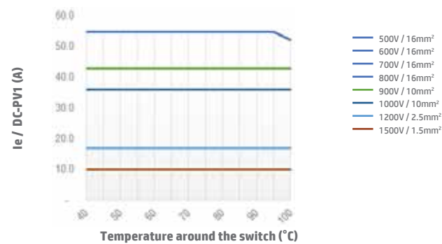
Switch SI55 2 poles DC-PV1 Open Type
