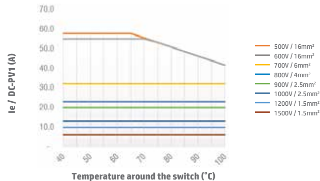
Switch SI32 2H DC-PV1 Open Type
