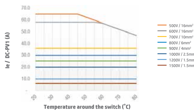
Switch SI38 2H DC-PV1 Enclosed Type
