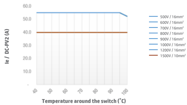
Switch SI55 4B/4S/4T DC-PV2 Open Type
