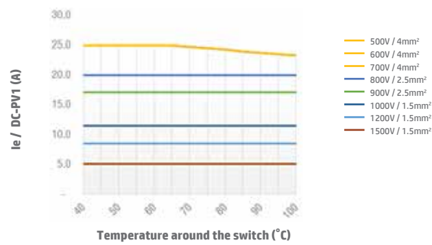
Switch SI25 2 poles DC-PV1 Open Type
