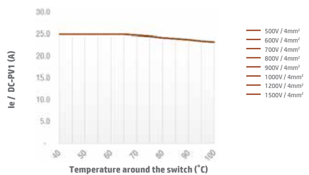
Switch SI25 4B/4S/4T DC-PV1 Open Type
