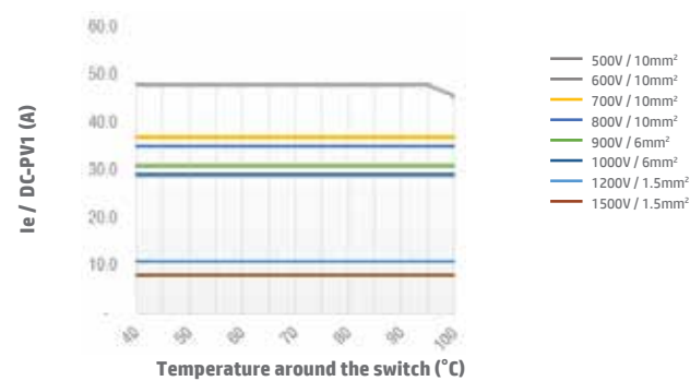
Switch SI40 2 poles DC-PV1 Open Type
