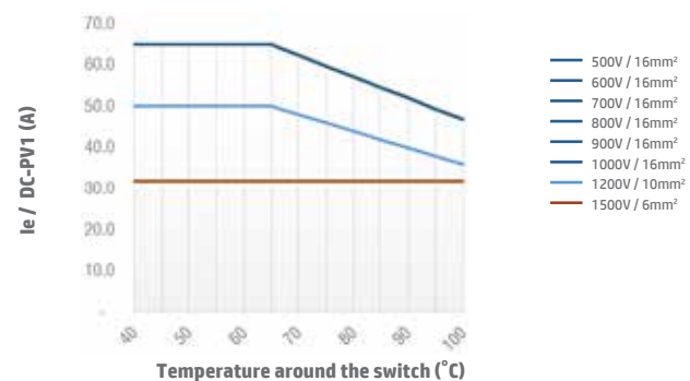
Switch SI38 4H DC-PV1 Open Type
