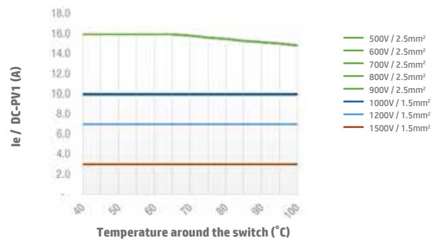
Switch SI16 2 poles DC-PV1 Open Type
