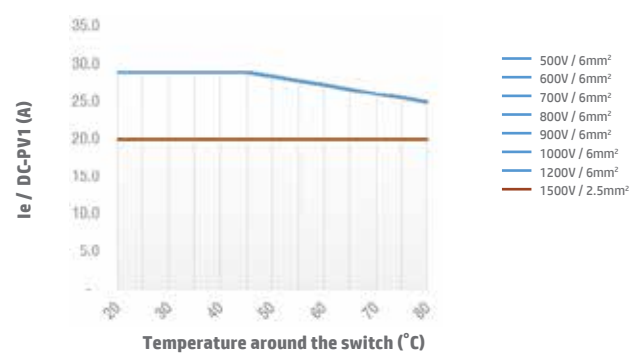
Switch SI16 4H DC-PV1 Enclosed Type
