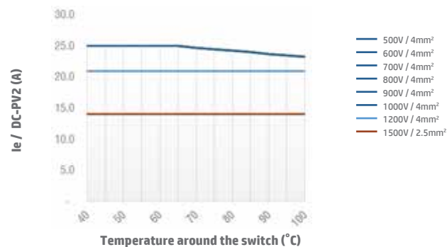
Switch SI25 4B/4S/4T DC-PV2 Open Type
