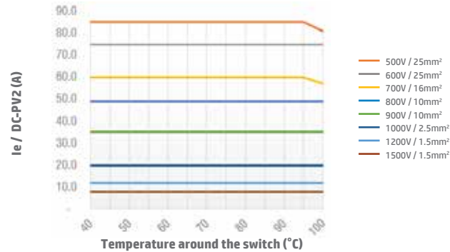
Switch SI55 2H DC-PV2 Open Type
