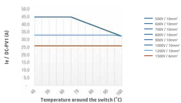
Switch SI25 4H DC-PV1 Open Type
