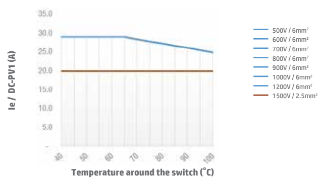
Switch SI16 4H DC-PV1 Open Type
