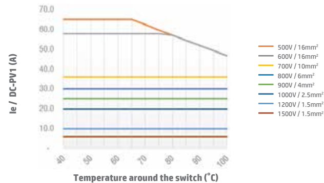
Switch SI38 2H DC-PV1 Open Type
