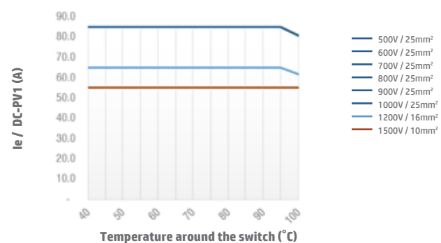
Switch SI55 4H DC-PV1 Open Type
