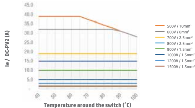
Switch SI25 2H DC-PV2 Open Type
