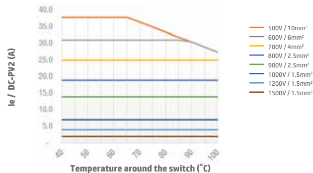
Switch SI38 2 poles DC-PV2 Open Type
