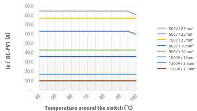
Switch SI55 2H DC-PV1 Open Type
