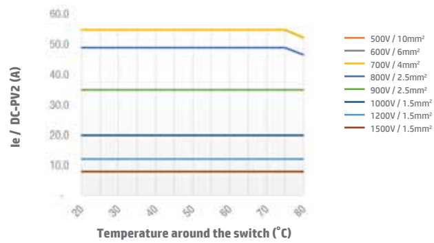
Switch SI55 2 poles DC-PV2 Enclosed Type
