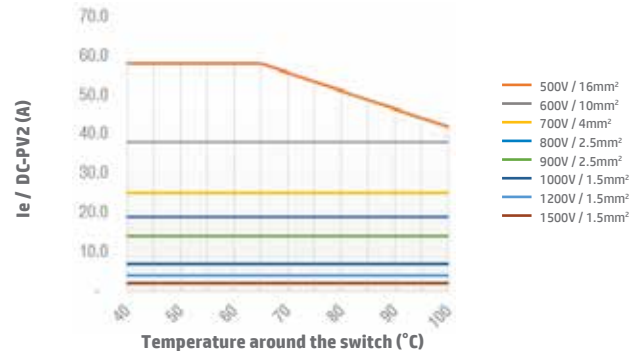
Switch SI38 2H DC-PV2 Open Type
