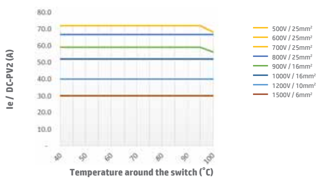
Switch SI40 4H DC-PV2 Open Type
