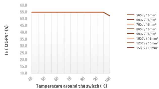
Switch SI55 4B/4S/4T DC-PV1 Open Type
