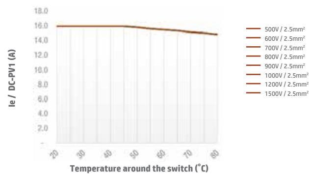
Switch SI16 4B/4S/4T DC-PV1 Enclosed Type
