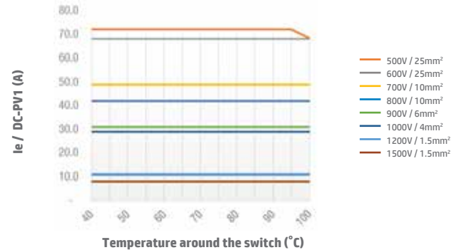
Switch SI40 2H DC-PV1 Open Type
