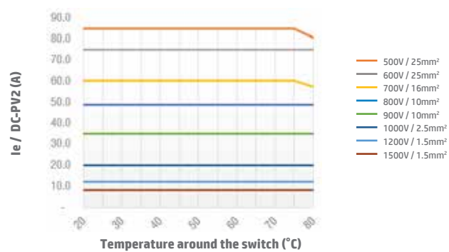
Switch SI55 2H DC-PV2 Enclosed Type
