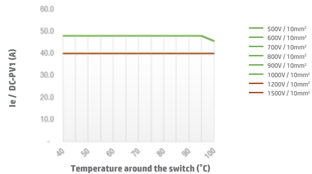
Switch SI40 4B/4S/4T DC-PV1 Open Type
