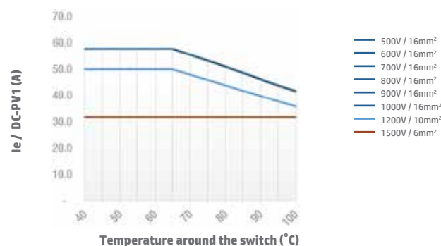
Switch SI32 4H DC-PV1 Open Type
