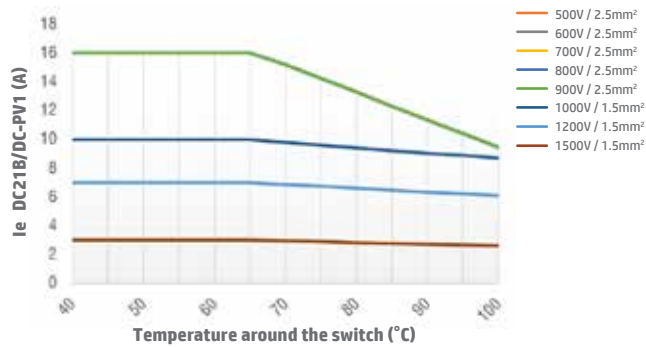
Switch SIM(E)16 2 poles all types except PEL64R
