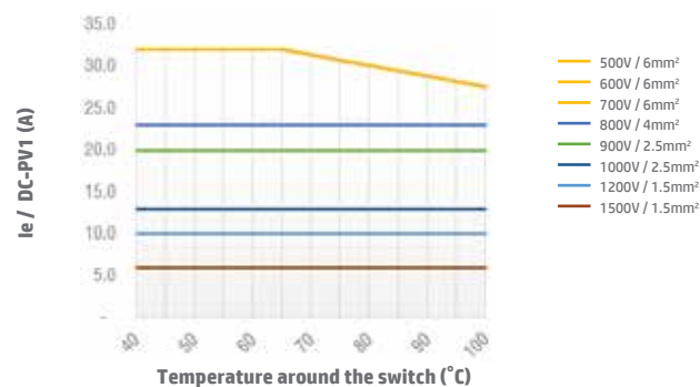
Switch SI32 2 poles DC-PV1 Open Type
