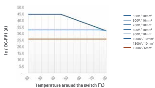
Switch SI25 4H DC-PV1 Enclosed Type
