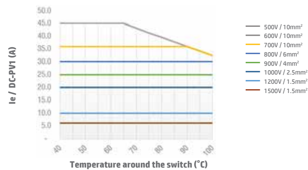
Switch SI38 2 poles DC-PV1 Open Type
