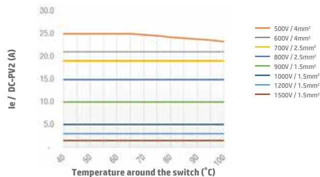
Switch SI25 2 poles DC-PV2 Open Type
