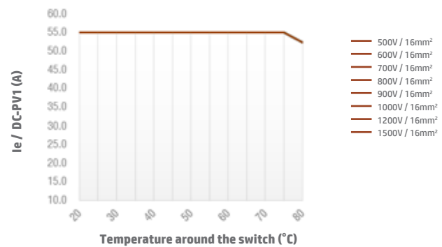
Switch SI55 4B/4S/4T DC-PV1 Enclosed Type
