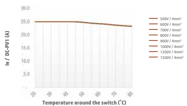
Switch SI25 4B/4S/4T DC-PV1 Enclosed Type
