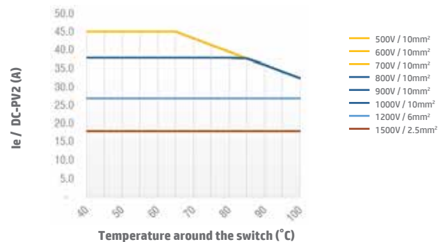
Switch SI38 4B/4S/4T DC-PV2 Open Type
