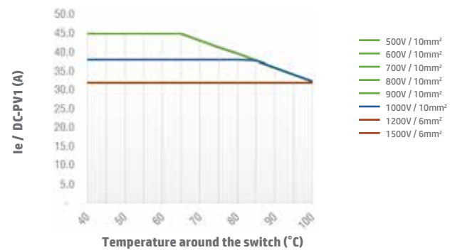
Switch SI38 4B/4S/4T DC-PV1 Open Type
