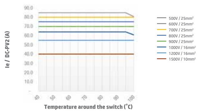
Switch SI55 4H DC-PV2 Open Type
