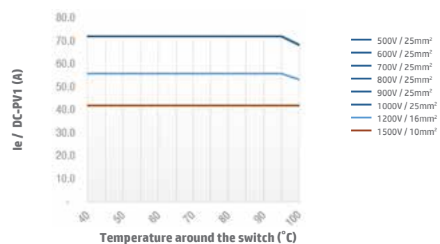
Switch SI40 4H DC-PV1 Open Type
