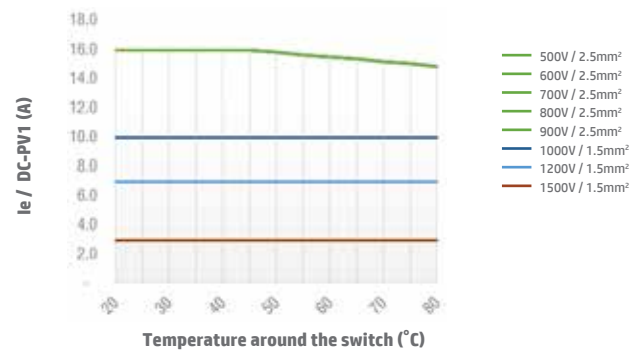
Switch SI16 2 poles DC-PV1 Enclosed Type
