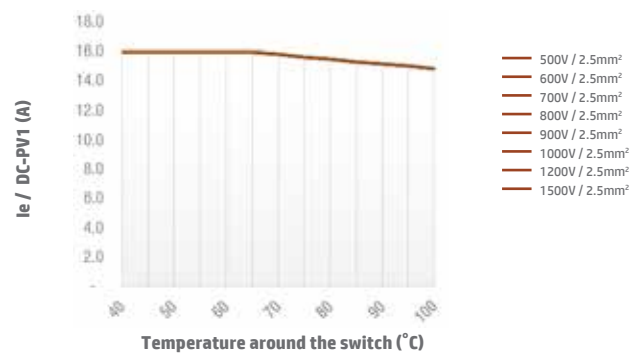
Switch SI16 4B/4S/4T DC-PV1 Open Type
