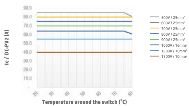
Switch SI55 4H DC-PV2 Enclosed Type
