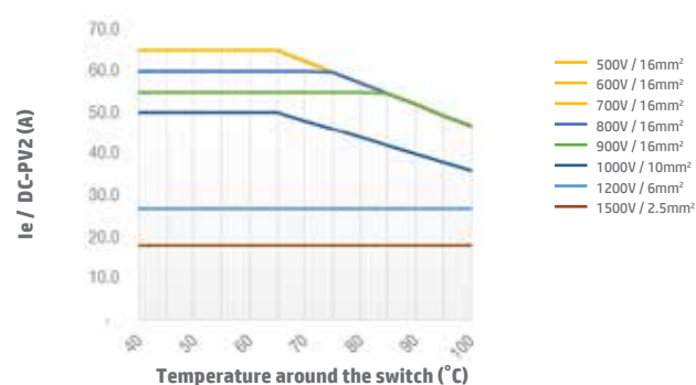
Switch SI38 4H DC-PV2 Open Type
