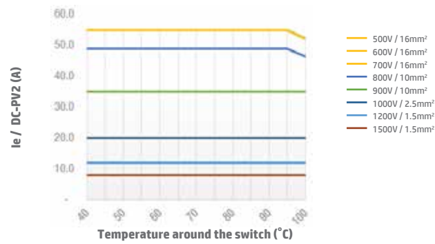
Switch SI55 2 poles DC-PV2 Open Type
