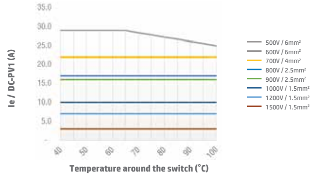
Switch SI16 2H DC-PV1 Open Type
