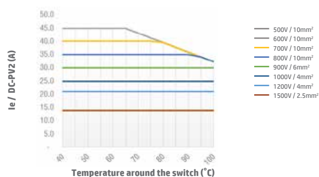
Switch SI25 4H DC-PV2 Open Type
