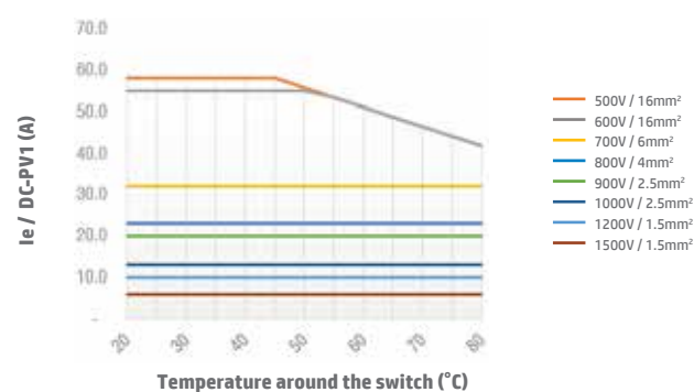
Switch SI32 2H DC-PV1 Enclosed Type
