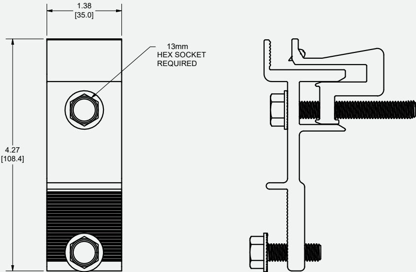
End Bracket
