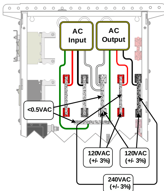
E-Panel with Left Hand Door
