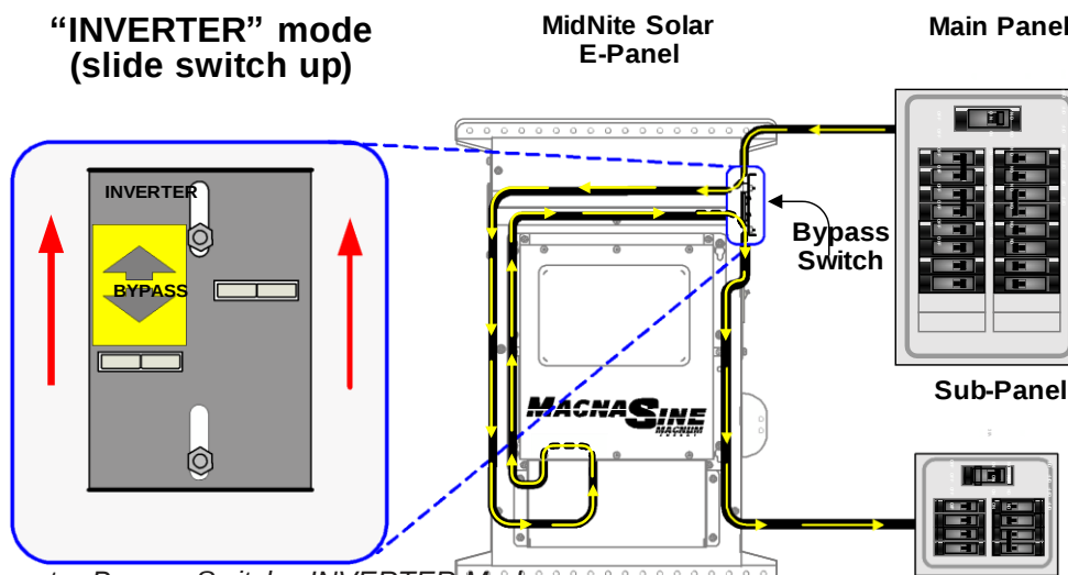
Figure 17, Inverter Bypass Switch - INVERTER Mode
