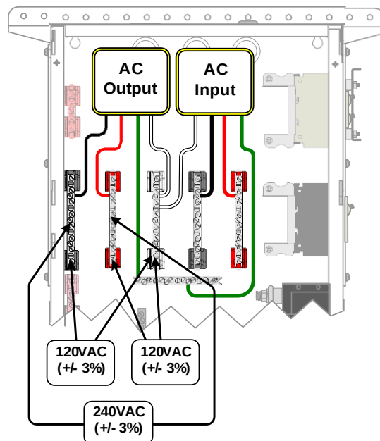
E-Panel with Right Hand Door
