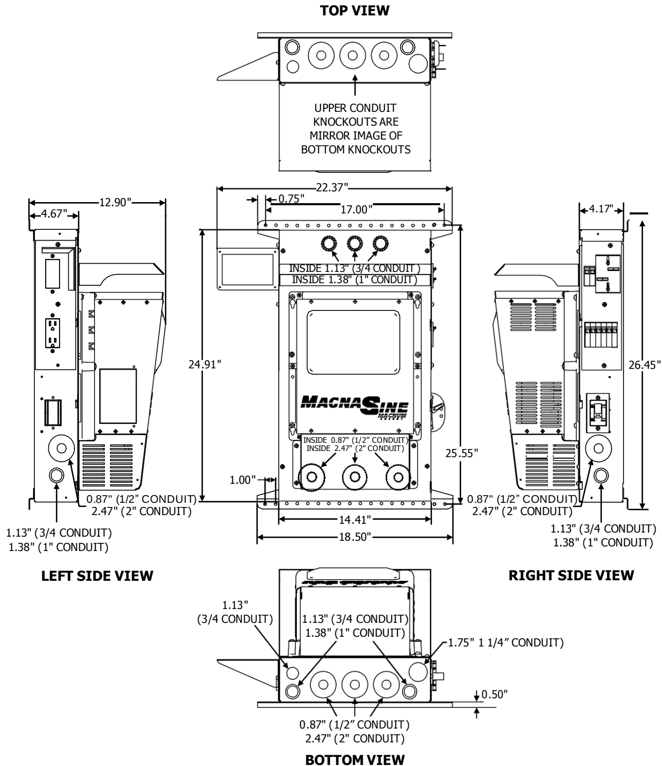
Figure 3, MNE-240 Series E-Panel Dimensions and Knockout Sizes
