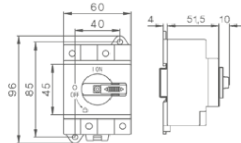
SI.. DBL with low height handle
