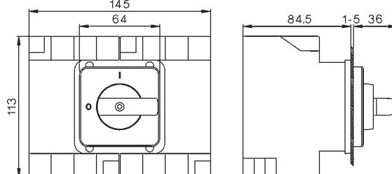
SI40PM / SI55PM 6, 3H, 8, 4H
