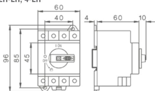
SI16DBL / SI25DBL / SI32DBL / SI38DBL with low height handle
