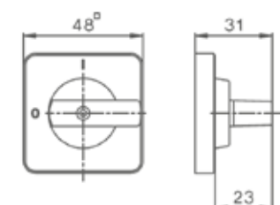
Lever Handle
