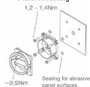
Panel Mounting
