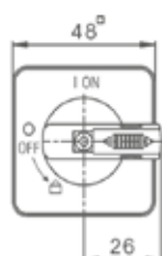
Lockable Lever
