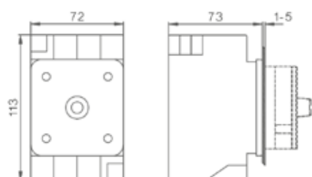
SI40PM / SI55PM 2, 2H, 4
