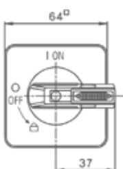
Lockable Lever
