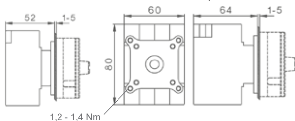
SI16PM / SI25PM / SI32PM / SI38PM 2, 2H, 4
