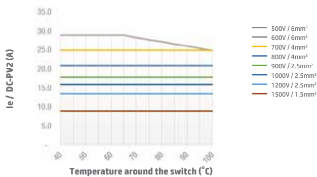
Switch SI16 4H DC-PV2 Open Type
