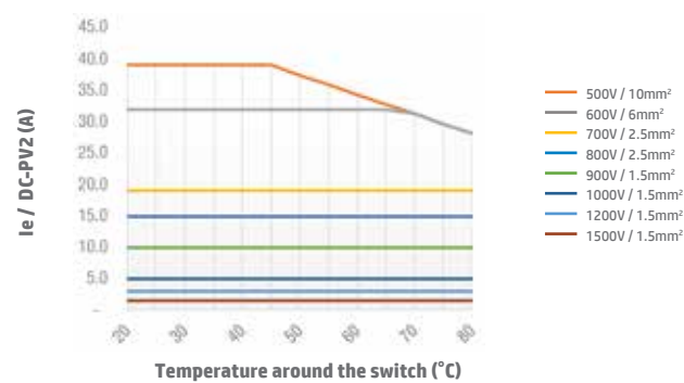
Switch SI25 2H DC-PV2 Enclosed Type
