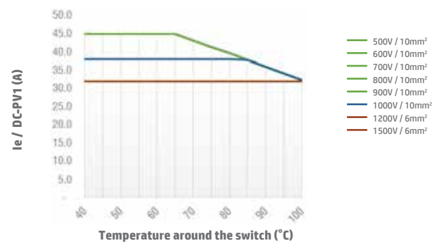
Switch SI38 4B/4S/4T DC-PV1 Open Type
