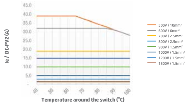
Switch SI25 2H DC-PV2 Open Type
