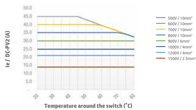
Switch SI25 4H DC-PV2 Enclosed Type
