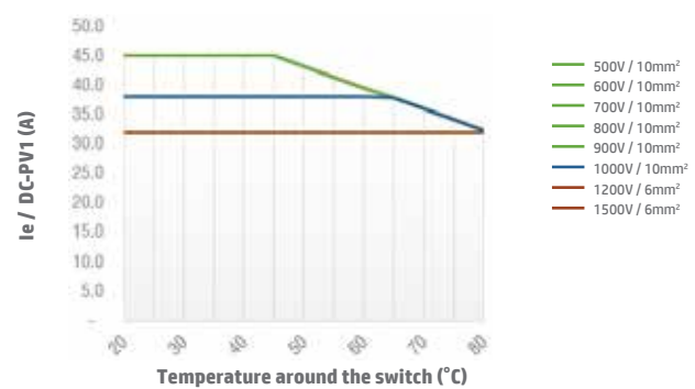
Switch SI38 4B/4S/4T DC-PV1 Enclosed Type
