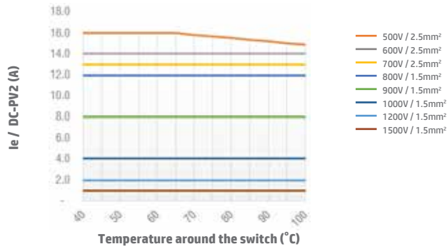
Switch SI16 2 poles DC-PV2 Open Type
