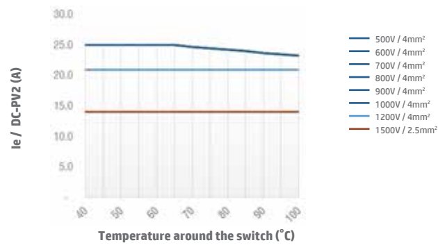
Switch SI25 4B/4S/4T DC-PV2 Open Type
