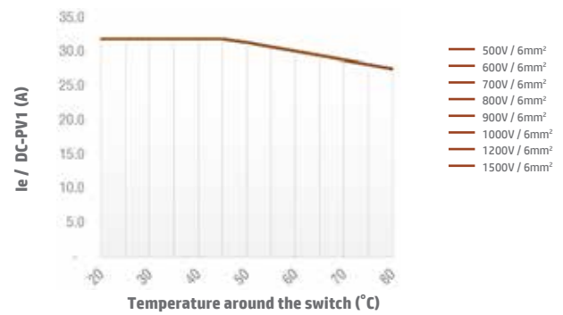
Switch SI32 4B/4S/4T DC-PV1 Enclosed Type
