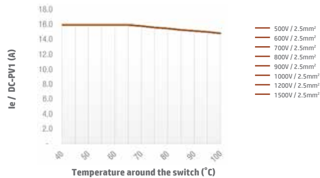
Switch SI16 4B/4S/4T DC-PV1 Open Type
