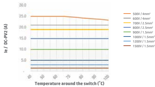
Switch SI25 2 poles DC-PV2 Open Type
