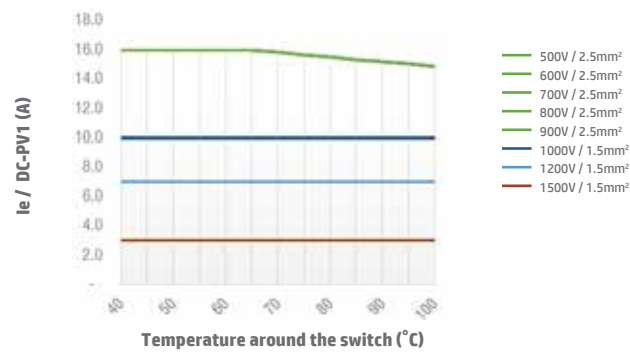
Switch SI16 2 poles DC-PV1 Open Type
