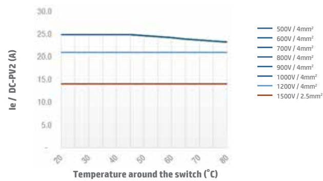
Switch SI25 4B/4S/4T DC-PV2 Enclosed Type
