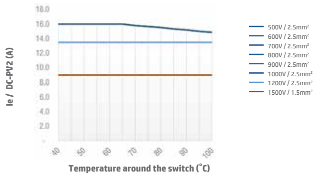
Switch SI16 4B/4S/4T DC-PV2 Open Type
