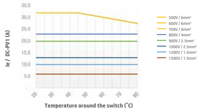
Switch SI32 2 poles DC-PV1 Enclosed Type
