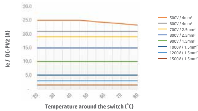
Switch SI25 2 poles DC-PV2 Enclosed Type
