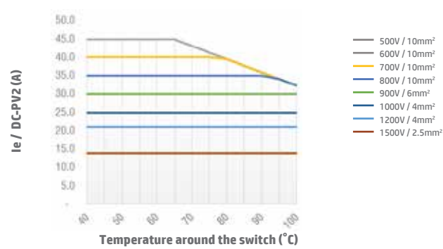
Switch SI25 4H DC-PV2 Open Type
