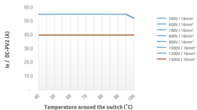
Switch SI55 4B/4S/4T DC-PV2 Open Type
