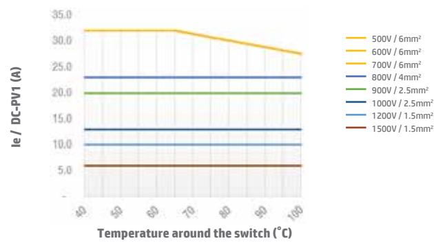
Switch SI32 2 poles DC-PV1 Open Type
