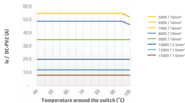
Switch SI55 2 poles DC-PV2 Open Type
