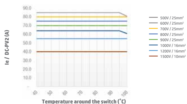
Switch SI55 4H DC-PV2 Open Type
