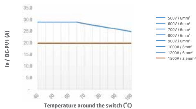
Switch SI16 4H DC-PV1 Open Type
