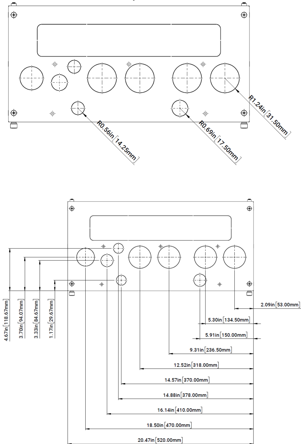
Top Plate
