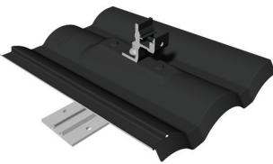
Ultra Rail W Tile Replacement with W Tile Hardware Kit
