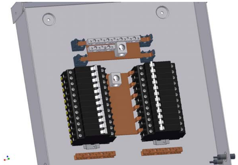
MNPV16 with bulkhead mount MC connectors
