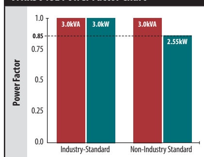
VFXR3048E Power Factor Chart
