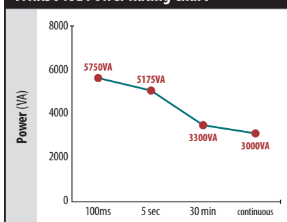
VFXR3048E Power Rating Chart
