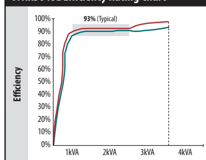
VFXR3048E Efficiency Rating Chart
