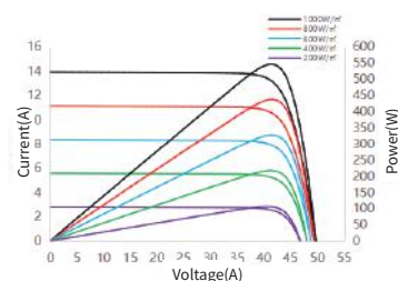
I-V/P-V Curve at Different Irradiation SS8-72HD-545M
