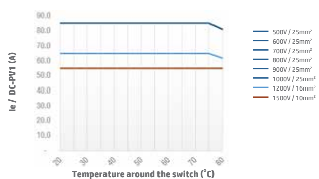
Switch SI55 4H DC-PV1 Enclosed Type
