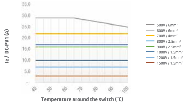
Switch SI16 2H DC-PV1 Open Type
