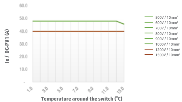
Switch SI40 4B/4S/4T DC-PV1 Enclosed Type
