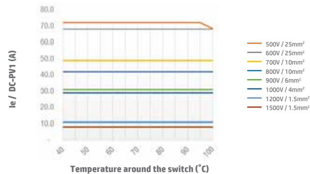
Switch SI40 2H DC-PV1 Open Type
