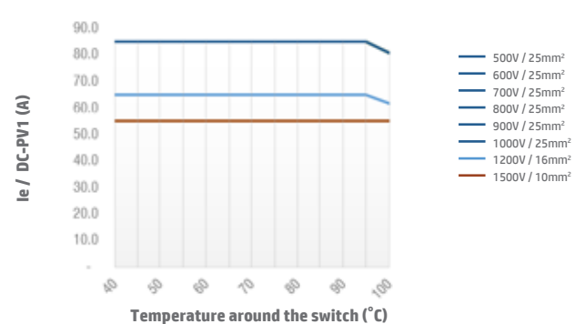
Switch SI55 4H DC-PV1 Open Type
