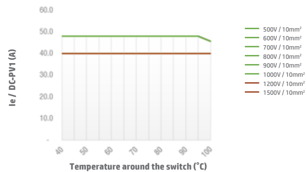
Switch SI40 4B/4S/4T DC-PV1 Open Type
