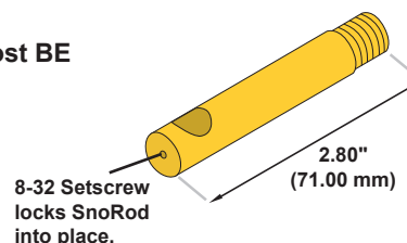
SnoPost B
