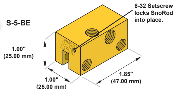
SnoPost BE
