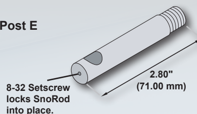
SnoPost
