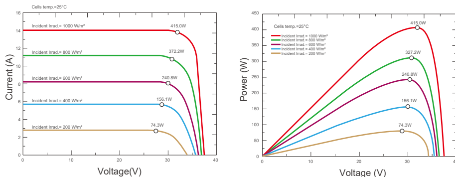
Current-Voltage & Power-Voltage Curves (RMH54-415B1)
