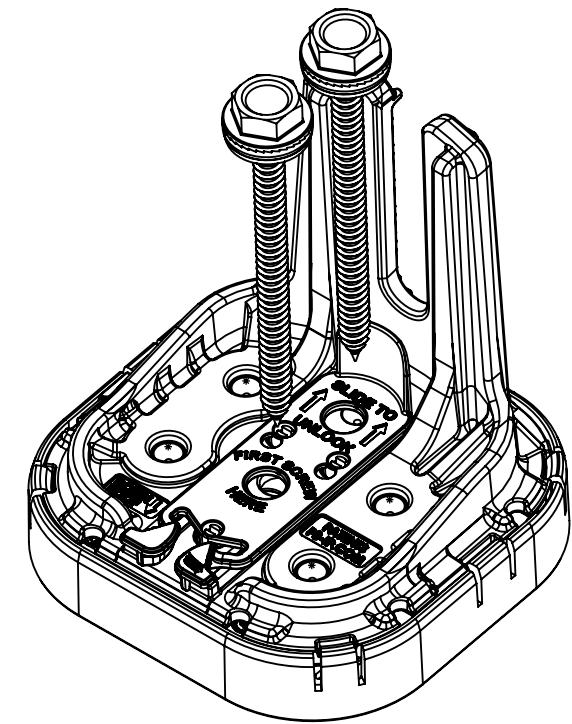
RAFTER ATTACH - 2 FASTENERS
