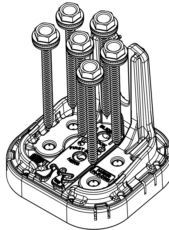
DECK ATTACH - 6 FASTENERS
