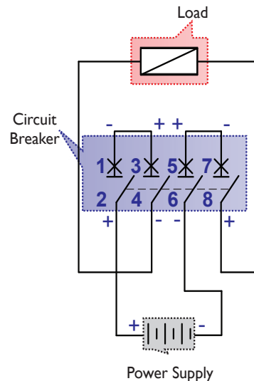
Figure 5: Four Pole, Double Break Isolates Load (400 Vdc, BU4) (300 Vdc / Pole)
