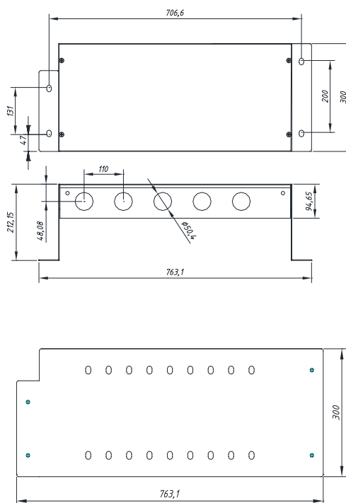
Optional: Post Mounting Plate
