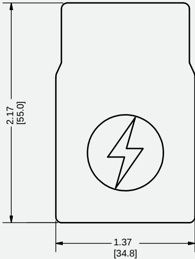
Rail End Cap, SMR100
