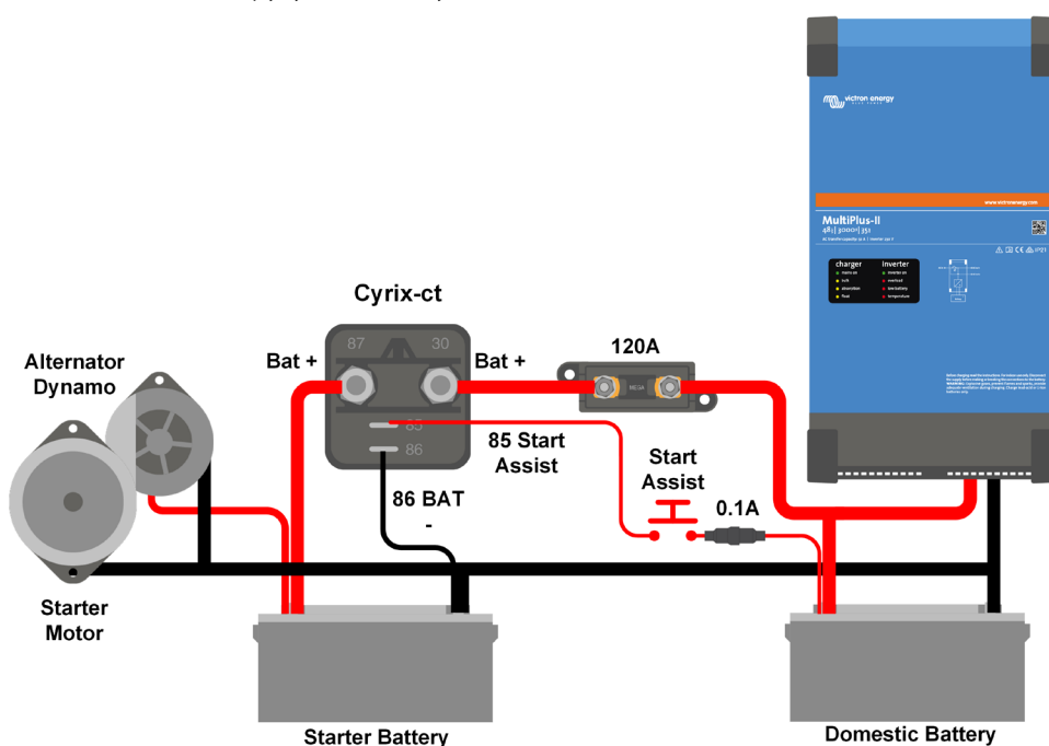
Cyrix-ct 12/24-120: connection diagram
