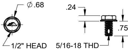
1) CAP SCREW, 5/16 x 3/4
