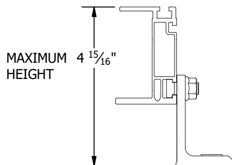
SOLARMOUNT HD ON L-FOOT
