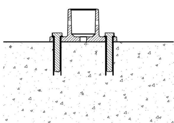
This cross section shows the mounting of a Post Base Plate to a precast concrete block.
