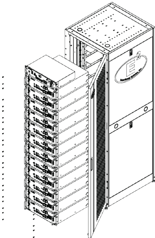
Exploded View Twelve-Battery with Control Unit Configuration
