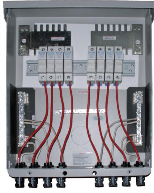
MNPV8 Factory wiring
