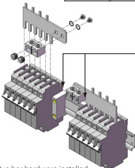
Bus bar hardware installed
