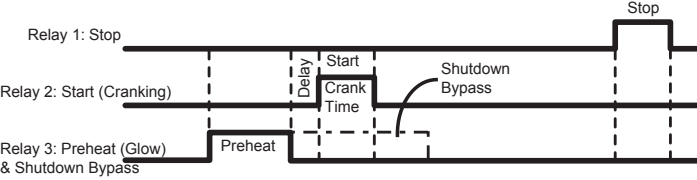
PulseStop Mode Timing Diagram for Gen Type 13
