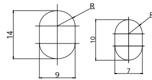
Mounting Hole
