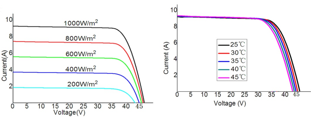
I-V Curves
